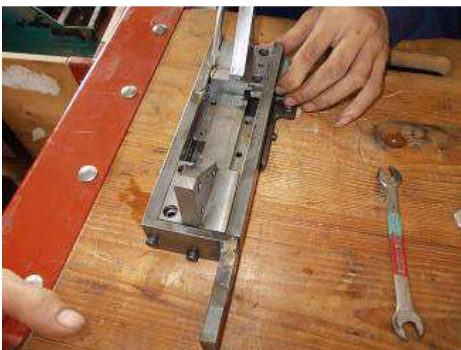
Photo 25: The gripper is mounted together again.
