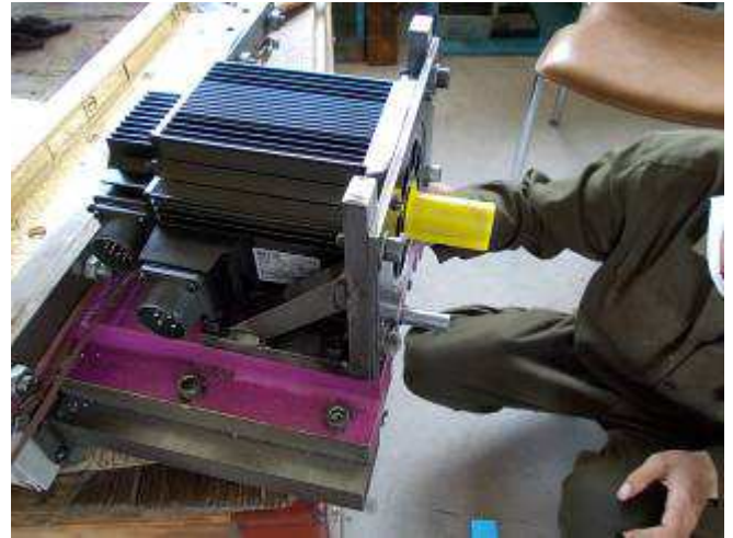
Photo 14: The X motor is now mounted on the cross slide.
